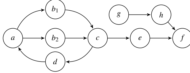
Figure 3. Weak and strong \sigma -support
