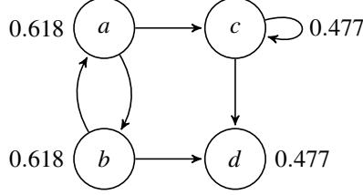
Figure 1. Example with Categoriser values
